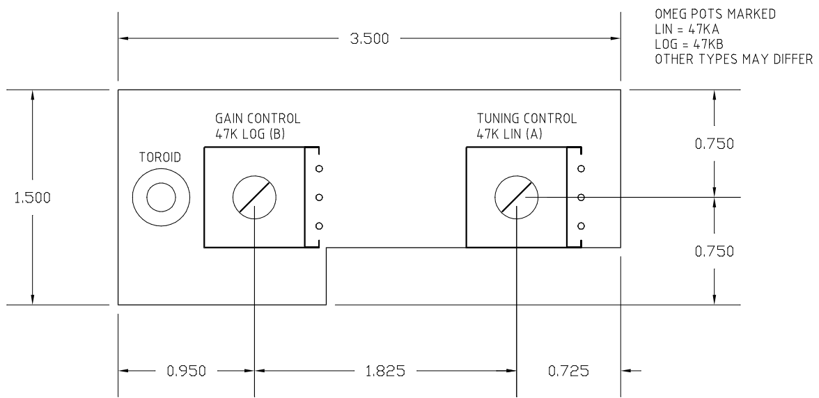
BOTTOM SIDE OF PCB
