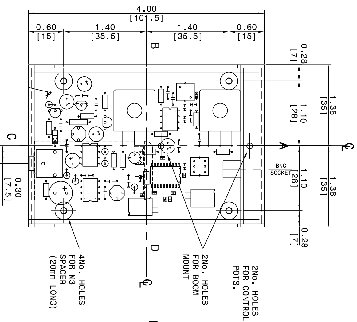
BASE PIECE PLAN
